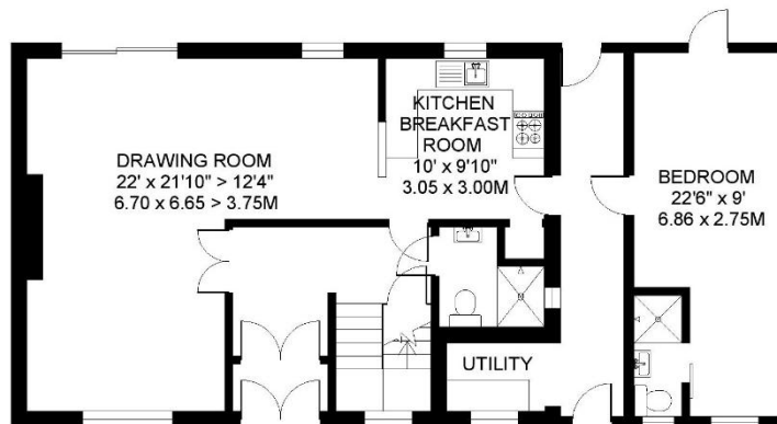
GROUND FLOOR 1037 SQ.FT.
